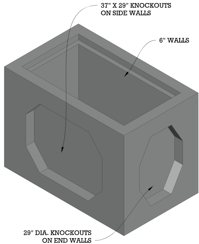
ISOMETRIC VIEW
