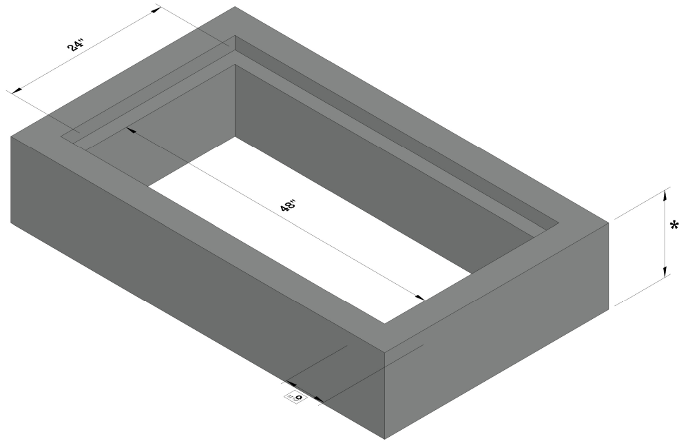
ISOMETRIC VIEW
